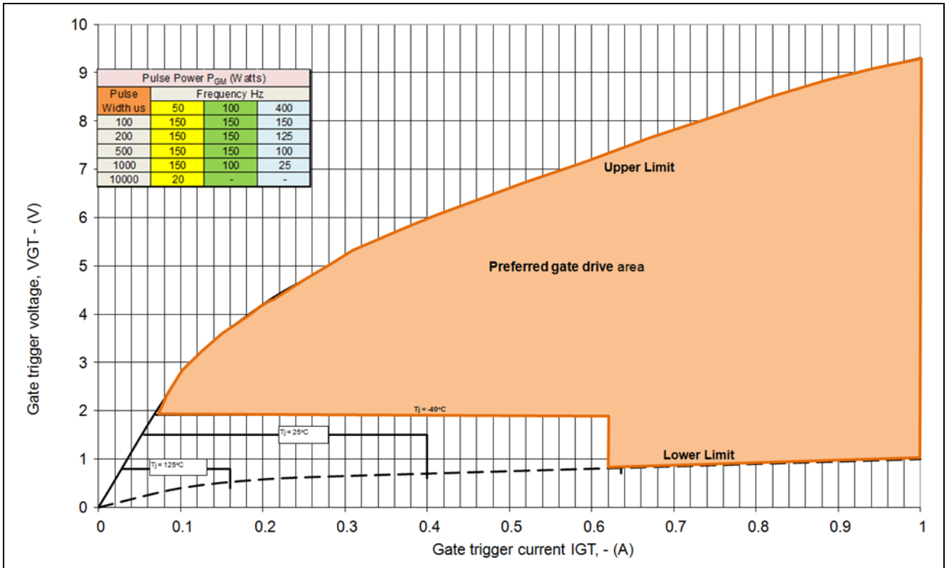
Fig. 14 Gate characteristics
