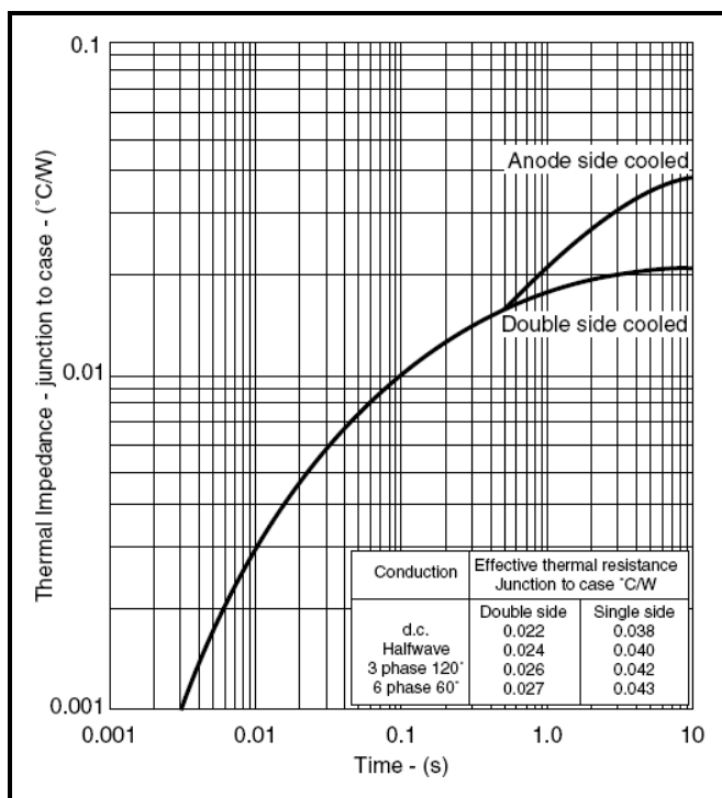
Fig.7 Maximum (limit) transient thermal impedance-junction to case
