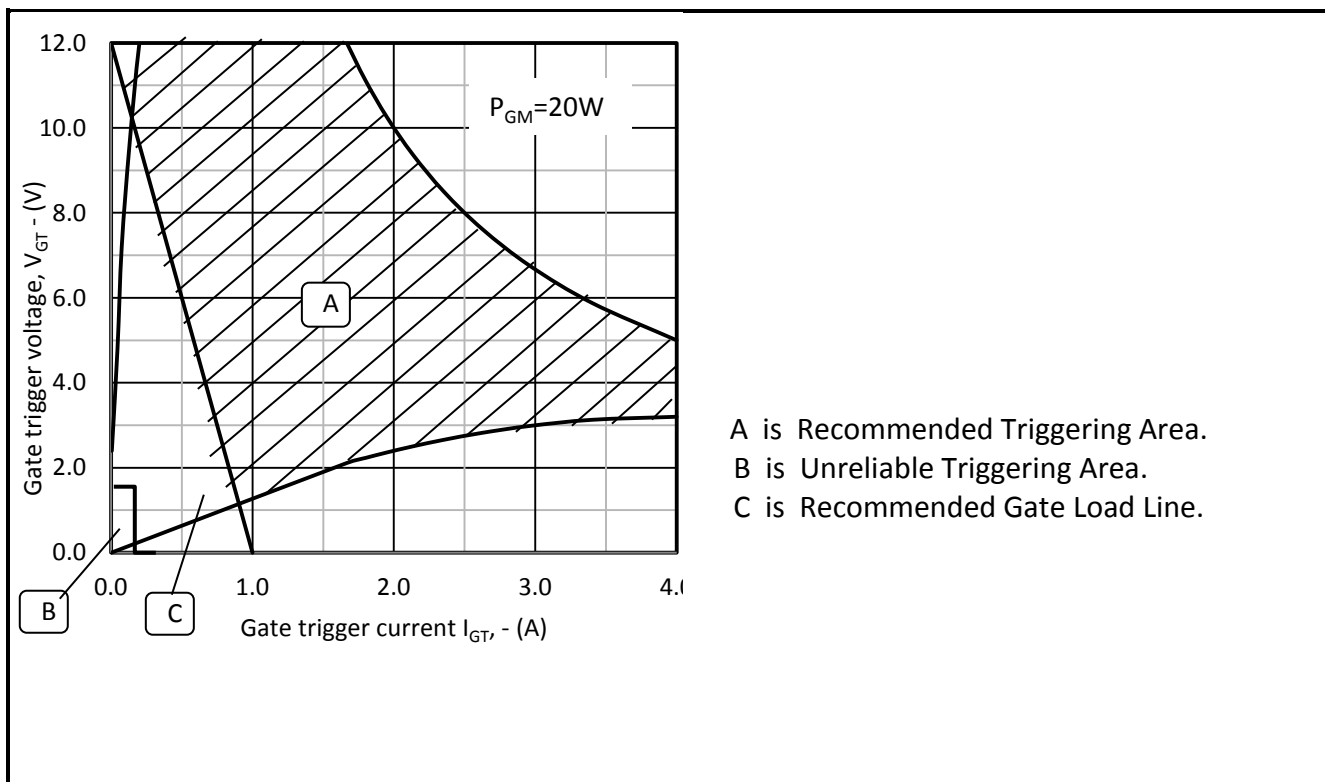
Fig.13 Gate characteristics
