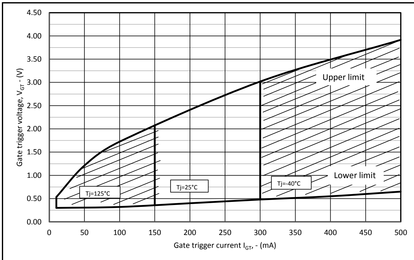
Fig.12 Gate characteristics
